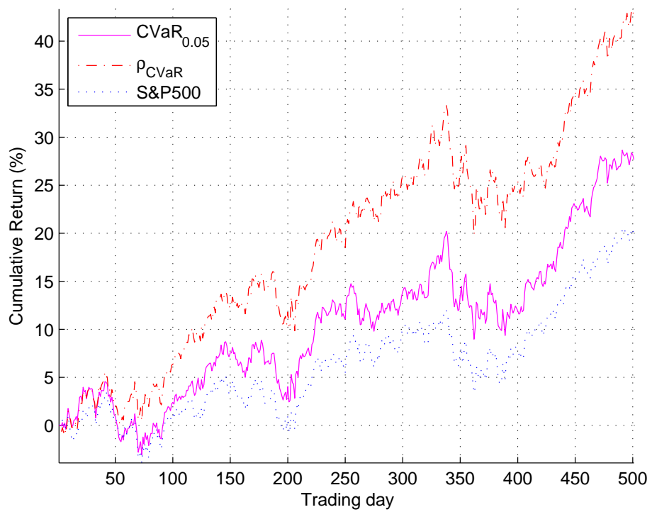
Figure 5: Aggregated out-of-sample cumulative returns against CVaR_{0.05} .
