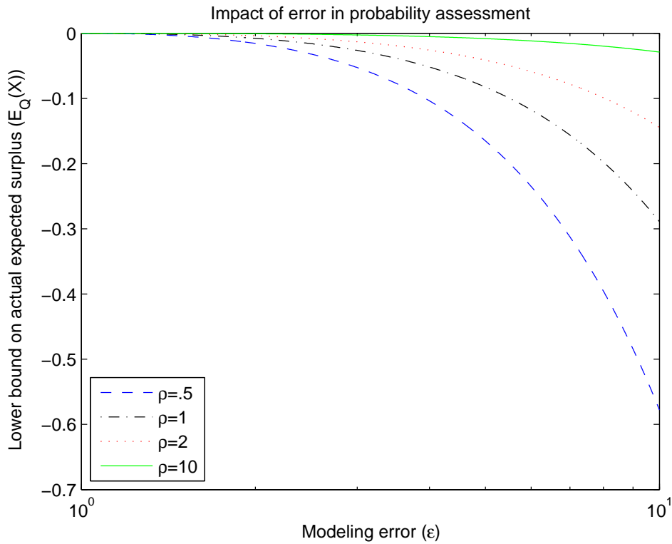
Figure 2: The impact of probability error on expected surplus for the debt management example.
