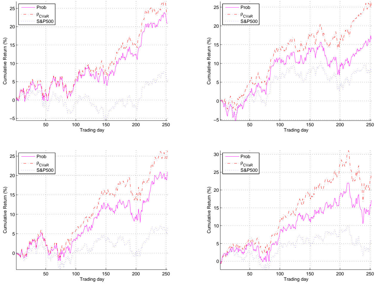
Figure 3: In-sample cumulative returns at various periods.
