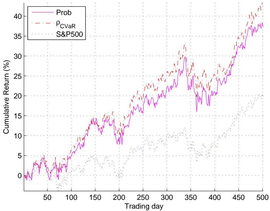
Figure 4: Aggregated out-of-sample cumulative returns.
