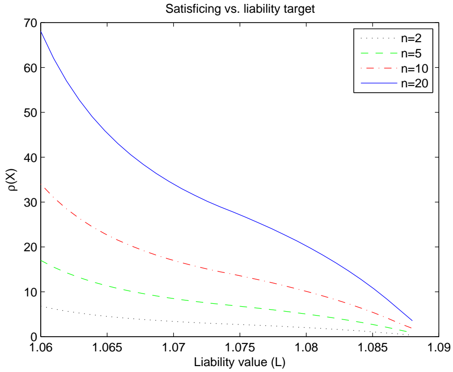
Figure 1: The effect of liability size on satisficing for the debt management example.
